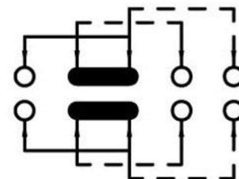
SCHEMATIC (SHORTING)
